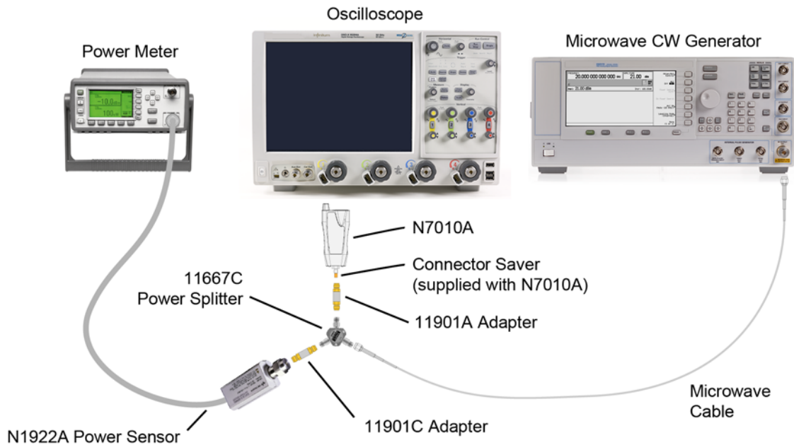
Figure 11 Bandwidth Test Setup
